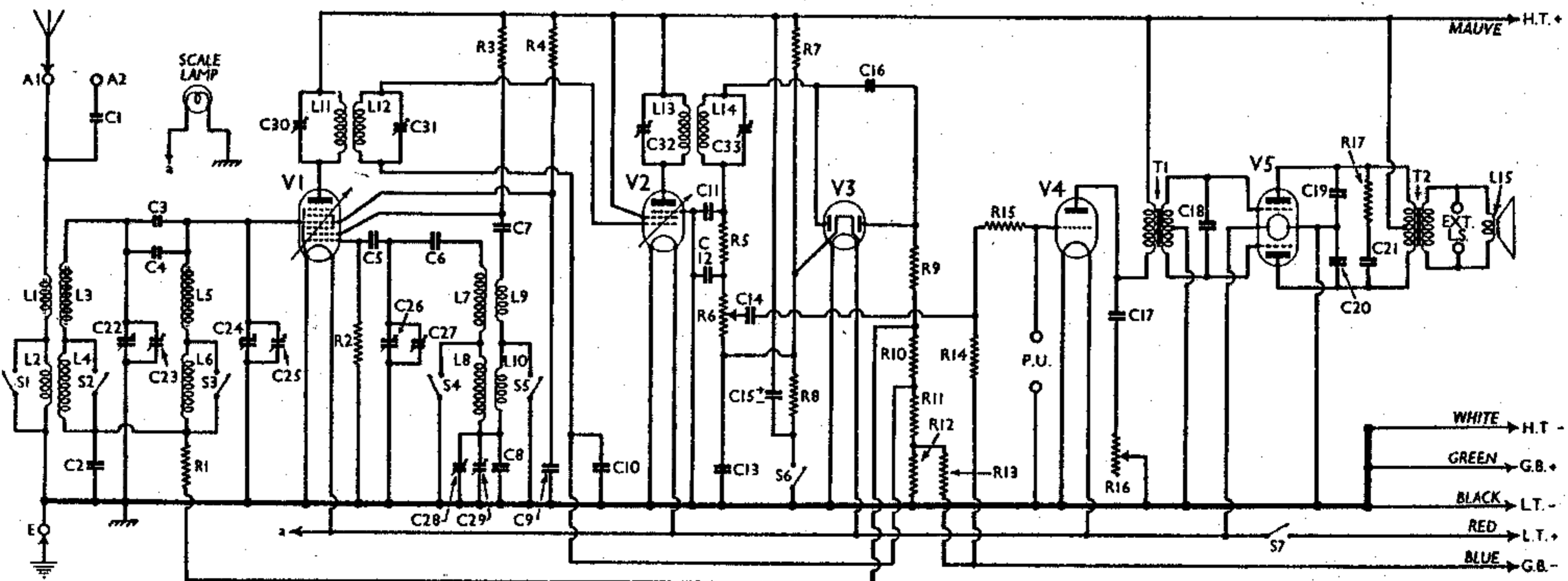
Circuit diagram of the Aerodyne 73 5-valve battery superhet. C3 and C4 are very small condensers, and only C3 may occur in some chassis. Where V1 is an FC2 (not FC2A ) there will be an extra small condenser between oscillator grid and pentode control grid of V1 .
